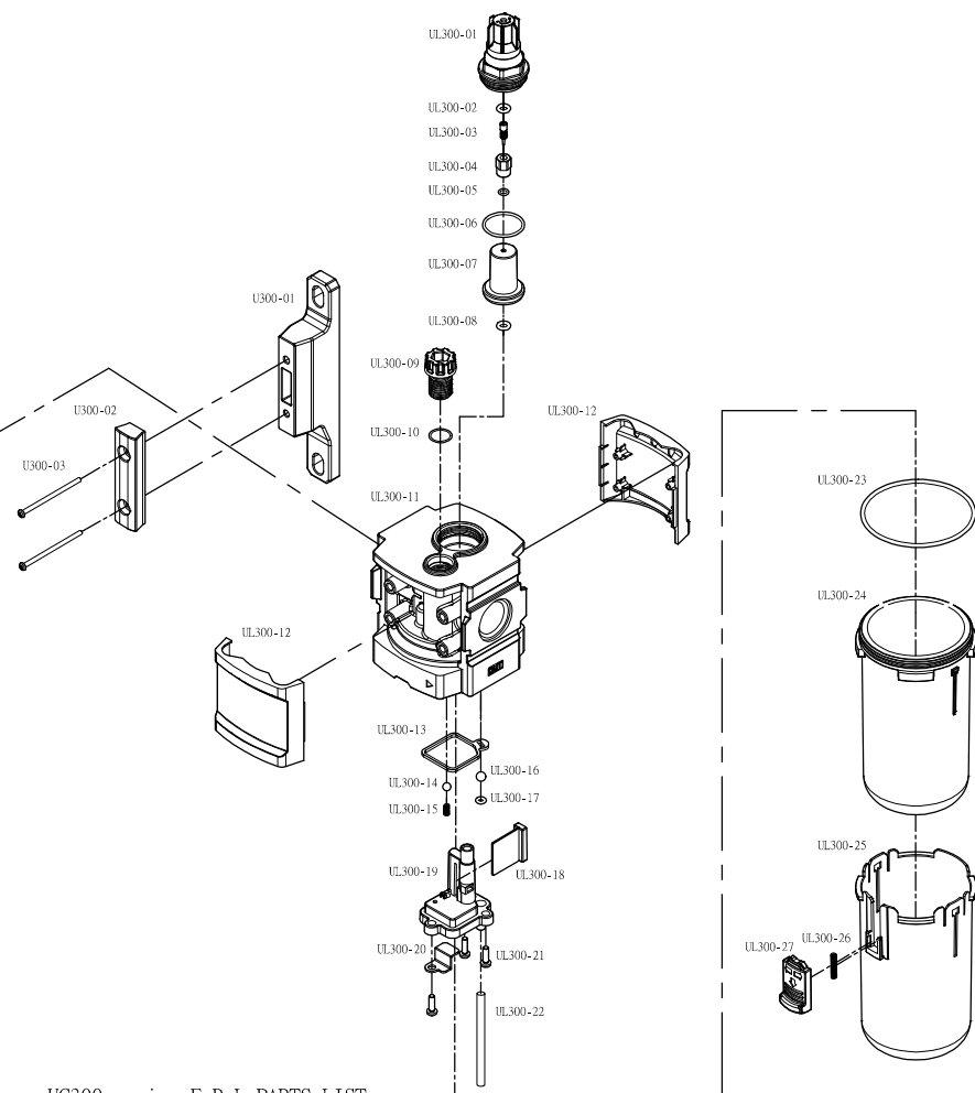
UC300 series F.R.L PARTS LIST
