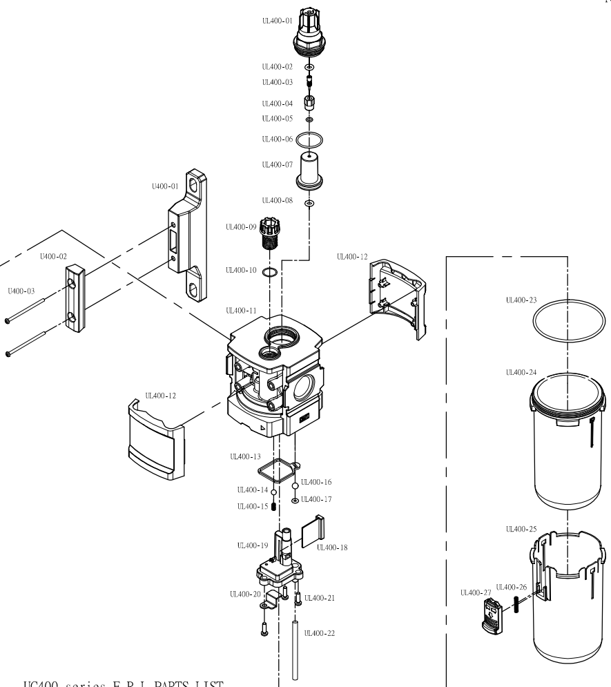
UC400 series F.R.L PARTS LIST
