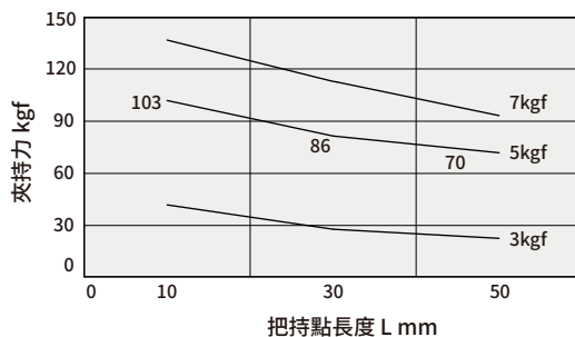
HCW、HCWL 60 - CLOSE
