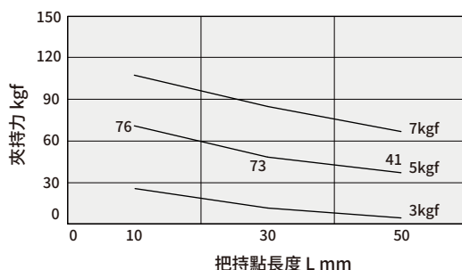
HCW、HCWL 44 - CLOSE
