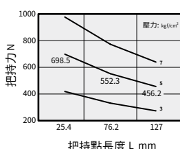
HDW 50 - CLOSE
