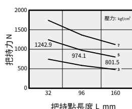
HDW 63 - OPEN
