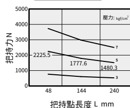
HDW 100 - OPEN
