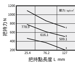
HDW 50 - OPEN
