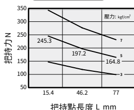
HDW 32 - CLOSE
