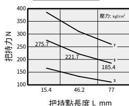
HDW 32 - OPEN
