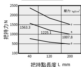
HDW 80 - OPEN
