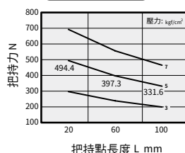
HDW 40 - OPEN
