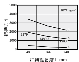
HDW 100 - CLOSE
