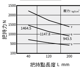
HDW 80 - CLOSE
