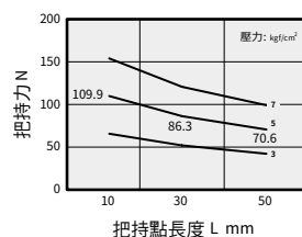
HDW 20 - CLOSE
